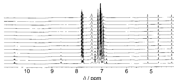
Figure 3. Time-evolved 1 H NMR spectra of the thermal rearrangement of 14d to 15d at 323 K in the C 6 D 6 . The bottom spectrum was recorded after heating for 1 h. The following spectra represent 2 h intervals with top spectrum corresponding to 27 h reaction time. For clarity, the signals from 0 to 4 ppm were omitted.
