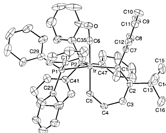
Figure 2. Molecular structure of iridabenzene 14d . The thermal ellipsoids are drawn at the 30% probability level. Selected bond lengths [Å] and bond angles [°]: Ir–P1 2.348(2), Ir–P2 2.306(3), Ir–C1 2.054(9), Ir–C5 2.000(9), Ir–C6 1.911(11), C1–C2 1.407(12), C2–C3 1.382(13), C3–C4 1.427(12), C4–C5 1.343(12), C1–C7 1.490(12), C2–C13 1.554(13); P1–Ir–P2 105.61(9), P1–Ir–C1 137.5(2), P2–Ir–C1 116.5(2), C5–Ir–C6 172.1(4), C1–Ir–C5 87.4(4), C1–Ir–C6 91.4(4), Ir–C1–C2 130.8(7), Ir–C1–C7 109.6(6), C1–C2–C3 119.5(9), C1–C2–C13 125.7(8), C2–C3–C4 128.2(9), C3–C4–C5 123.9(8), Ir–C5–C4 130.2(7), Ir–C6–O 174.1(8).
