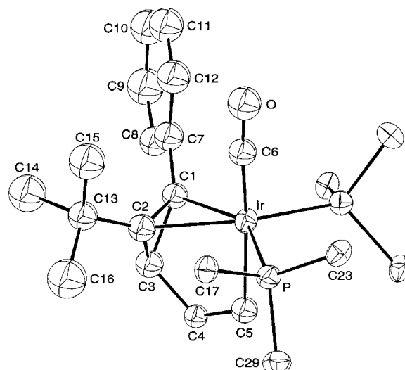
Figure 1. Molecular structure of iridabenzvalene 13d . The thermal ellipsoids are drawn at the 30% probability level. Only the ipso - \text{PPh}_3 carbon atoms are shown for clarity. Selected bond lengths [Å] and bond angles [°]: Ir–P 2.353(3), Ir–C1 2.19(2), Ir–C2 2.22(2), Ir–C5 2.18(3), Ir–C6 1.73(2), C1–C2 1.41(3), C1–C3 1.56(3), C1–C7 1.47(3), C2–C3 1.57(3), C2–C13 1.49(3), C3–C4 1.40(3), C4–C5 1.38(4); P–Ir–Pi 110.4(1), P–Ir–C2 136.4(5), Pi–Ir–C1 146.6(5), C1–Ir–C2 37.1 (6), C5–Ir–C6 174(1), C1–Ir–C5 81.5(8), C2–Ir–C5 80.4(8), C3–C1–C7 130(2), C3–C2–C13 129(2), C1–C3–C2 54(1), C3–C4–C5 115(2), C4–C5–Ir 111(2).
